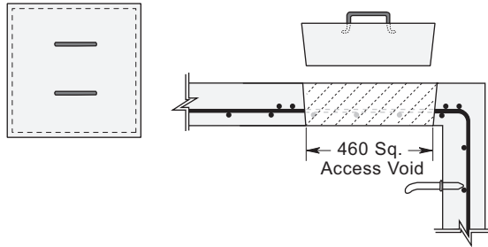
Tapered Type
