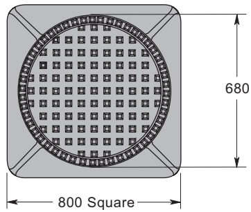
Tapered Type
