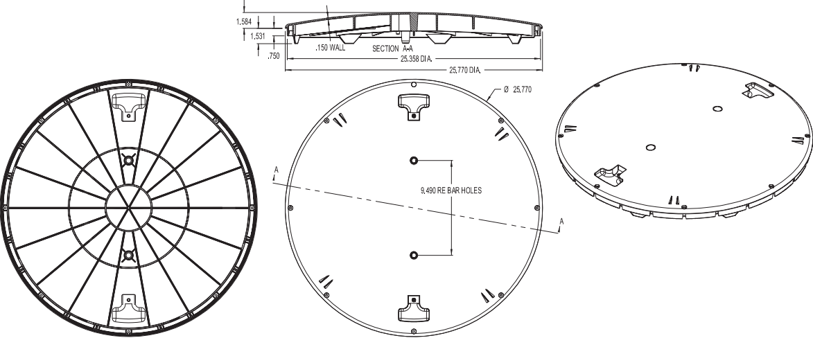
POLYLOK 24" COVER PART NO. 3008-RC MATERIAL - HDPE
