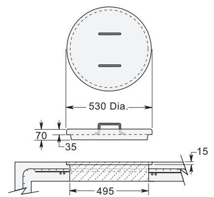
Precast Concrete Hatch Cover
