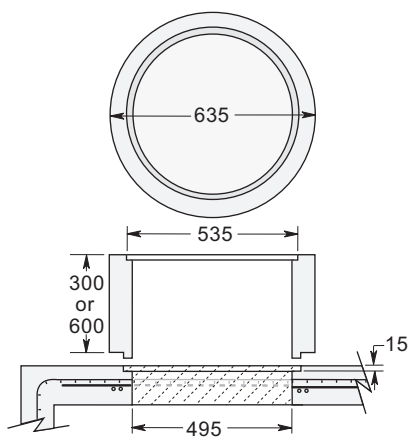
Precast Concrete Access Extension
