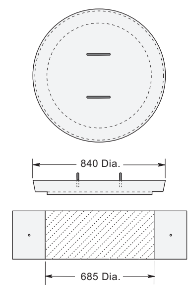
Precast Concrete Hatch Cover
